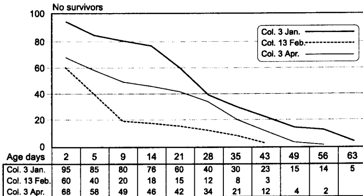
Fig. 1 Survival of A. dorsata workers in A. mellifera colonies. In January and February, brood combs with emerging A. dorsata workers was introduced into A. mellifera colonies Nos 3 and 13. In April, A. dorsata workers which emerged in incubator were introduced into A. mellifera colony No. 3 in large wire mesh cage.
